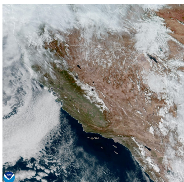
13 Feb 2026 22:41Z - NOAA/NESDIS/STAR GOES-West - GEOCOLOR Composite - Pacific Southwest
