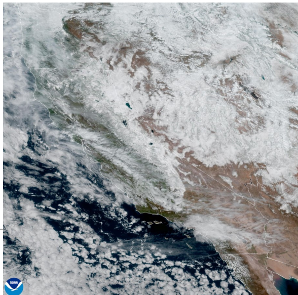
20 Feb 2026 19:36Z - NOAA/NESDIS/STAR GOES-West - GEOCOLOR Composite - Pacific Southwest
